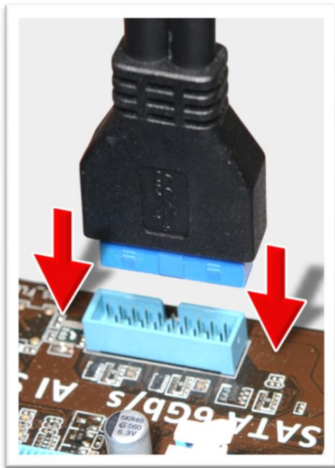
Motherboard
